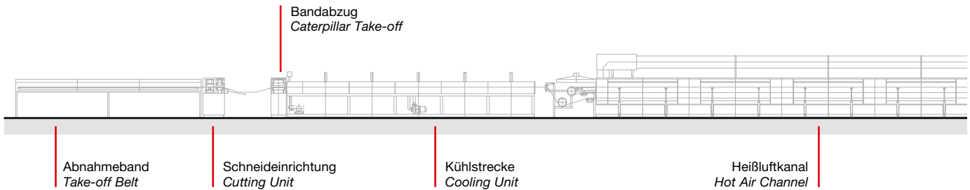
Kompaktextruder GSC Vak 90/k-20D Compact extruder GSC Vak 90k-20D
